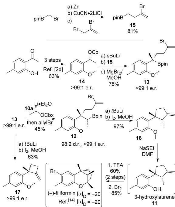
Scheme 6. Total synthesis of (–)-filiformin. TFA=trifluoroacetic acid.
