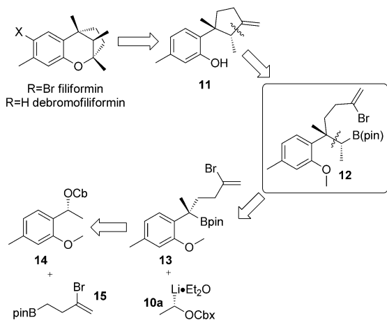
Scheme 5. Retrosynthetic analysis of (–)-filiformin.
